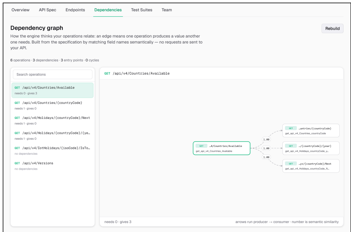
Figure 8.14: SPDG Visualization
