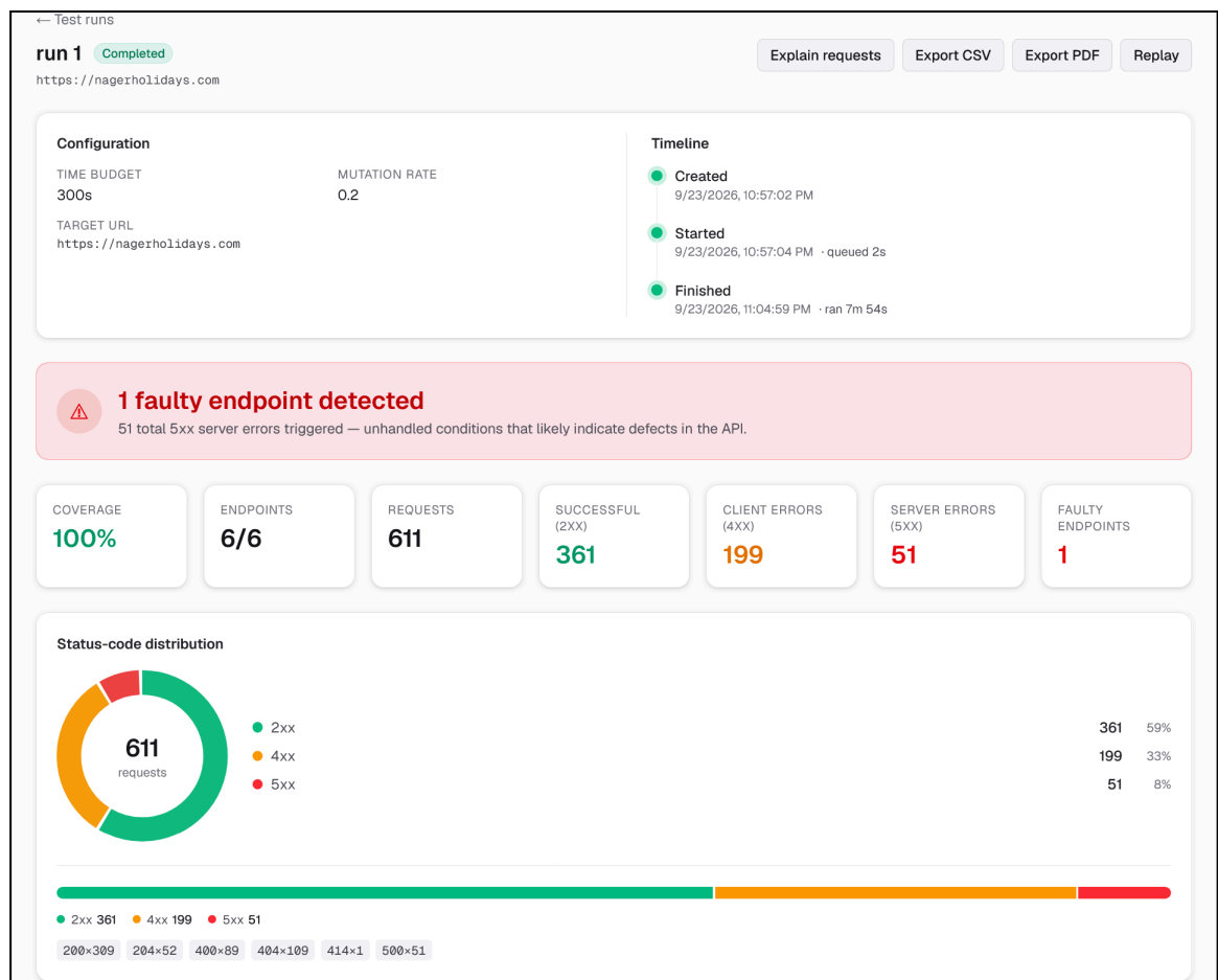
Figure 8.16: Test report
