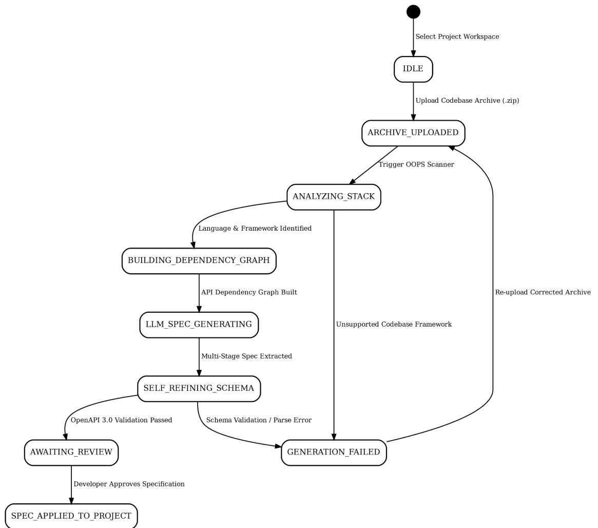
Figure 5.3: State Transition for Automated API Spec generation
