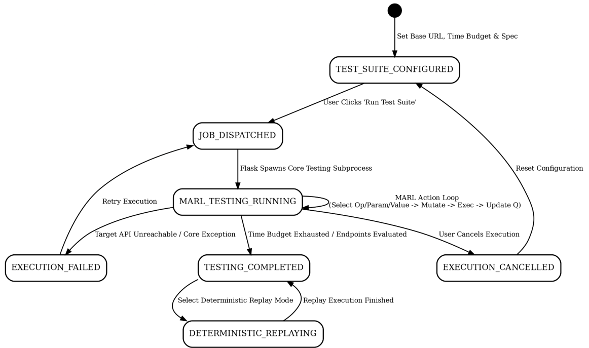
Figure 5.4: State Transition for Automated Test Suit Execution
