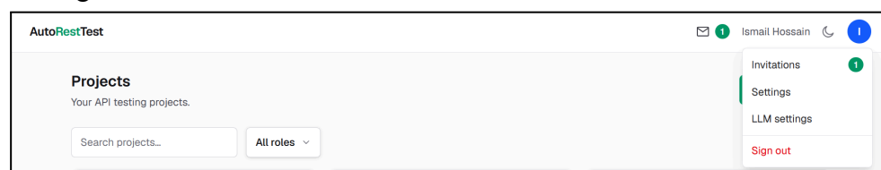
Figure 8.6: Navbar
