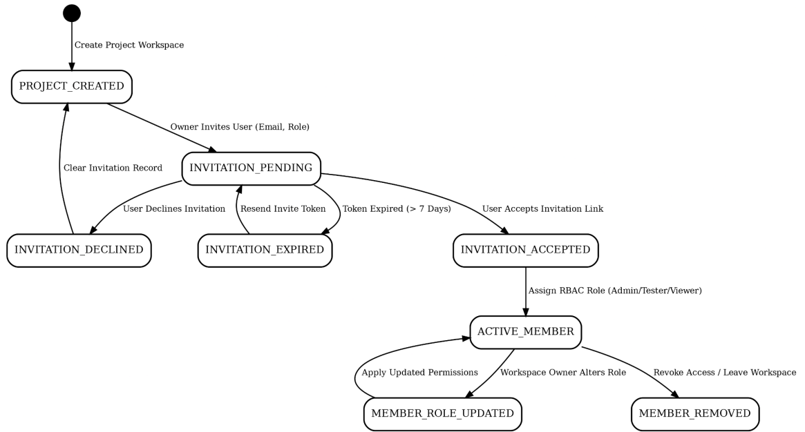
Figure 5.2: State Transition for Project Collaboration & Access Control
