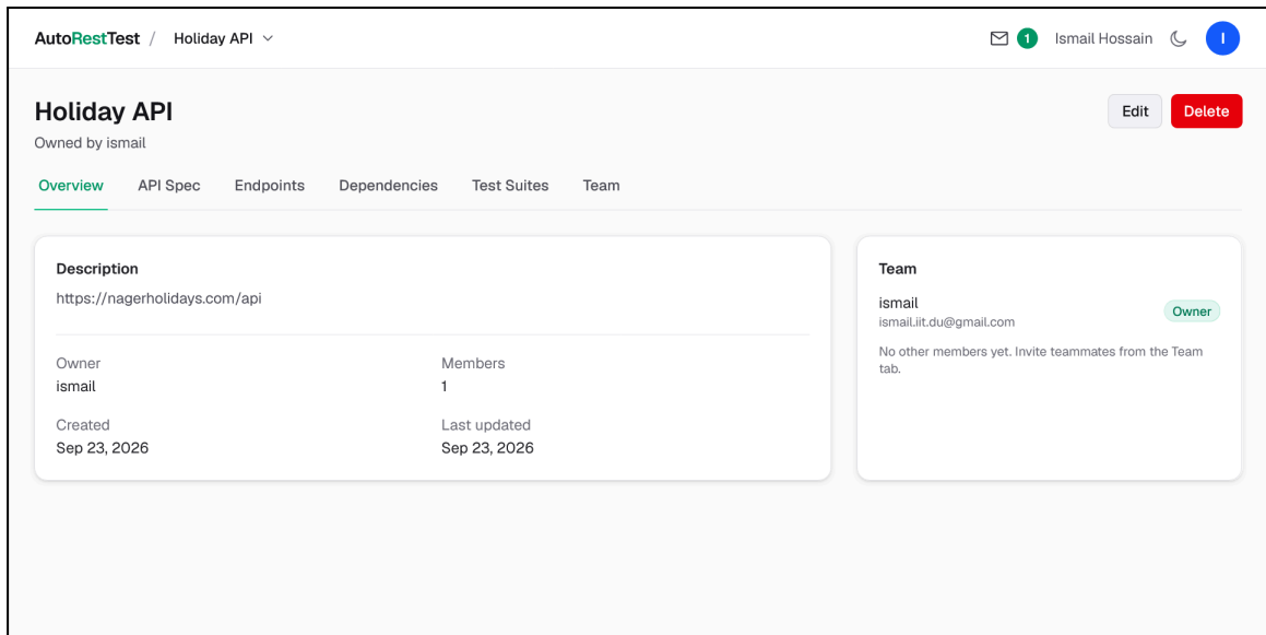
Figure 8.9: Project overview
