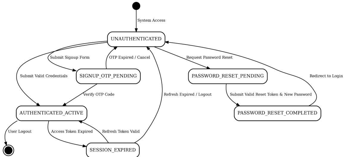
Figure 5.1: State Transition for Authentication and User Identity Lifecycle
