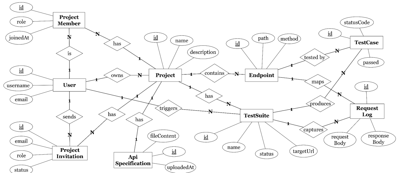
Figure 3.1: Entity Relationship Diagram
